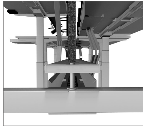
Easy cable tray installation No additional tools are required for assembly.
